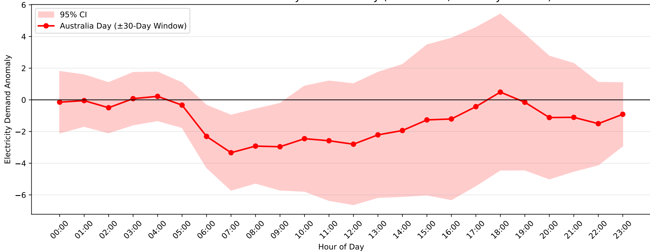
Meadowbank Demand Anomaly: Australia Day (2004-2017, \pm 30 -Day Window)
